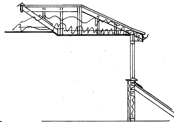
SECTION 1:50
